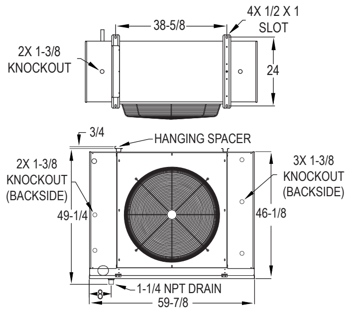
Figure 1 - Single Fan
